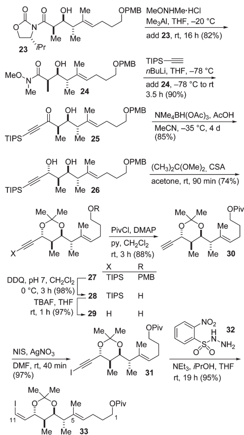
Scheme 4. Preparation of Vinyl Iodide 33 (C1–C11 Fragment)
