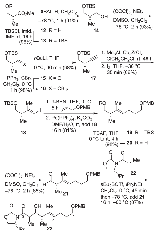
Scheme 3. Preparation of Aldol Product 23 (C1–C9 Fragment)
