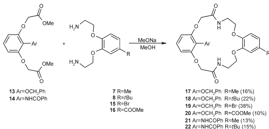
Scheme 4. Synthesis of diazacoronands possessing planar chirality.
