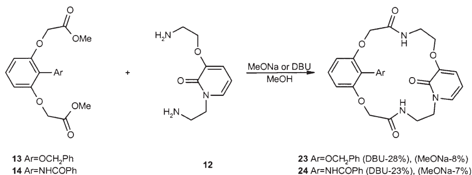
Scheme 6. Synthesis of chiral diazacoronands containing the pyridin-2-one moiety.
