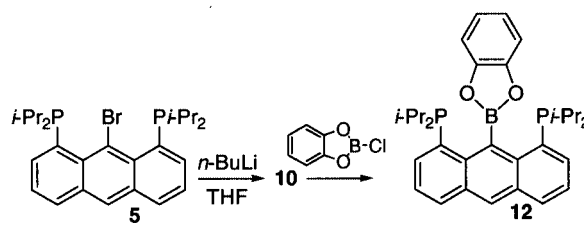
Scheme 2. Introduction of a boron substituent.
