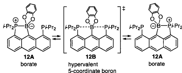
Scheme 3. Very rapid P-B bond switching equilibrium in 12 .
