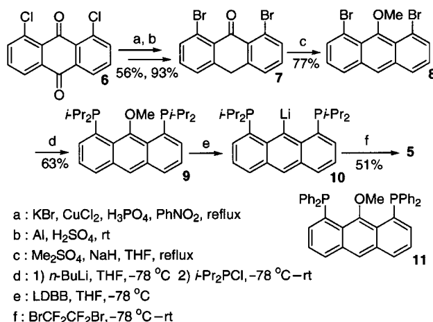
Scheme 1. Synthesis of 5 .
