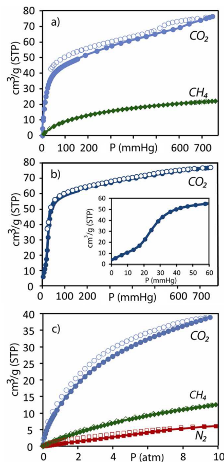
Figure 5. (a) Adsorption/desorption isotherms for \text{CO}_2 and \text{CH}_4 onto porous AgL-B at 195 K. (b) \text{CO}_2 adsorption/desorption isotherm for the porous AgL-P compound at 195 K. Inset, enlargement of the low pressure region. (c) Adsorption/desorption isotherms for \text{CO}_2 , \text{CH}_4 and \text{N}_2 onto AgL-B at room temperature and up to 10 atm.
