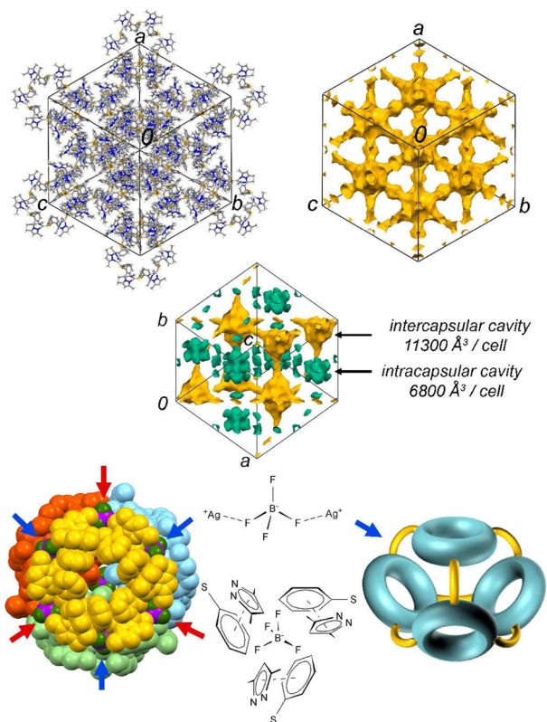
Figure 2. Above, crystal packing of AgL-B depicting the rigid part of the structure in stick and the cavities in yellow. Middle, the two different types of cavities are depicted in yellow and green, respectively. Below, description of the supramolecular contacts between the \text{BF}_4^- anions and the hexameric moieties.
