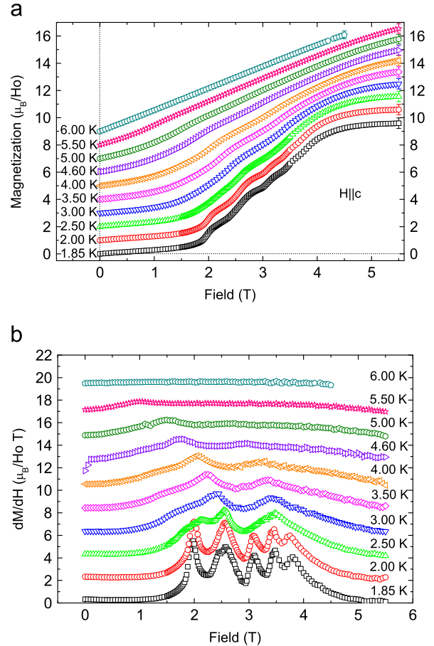
Fig. 4. (Color online) (a) Magnetization measurements with the data shifted by 1 \mu_B between different temperatures. The low temperature data show a cascade of up to five transitions that disappear as the temperature is increased. (b) We plot the derivative of the magnetization with the magnetic field as a function of the magnetic field. Peaks correspond to transitions, providing the phase diagram discussed in the next figure. Derivative data have been shifted by 2 \mu_B/\text{Ho T} for the different temperatures.
