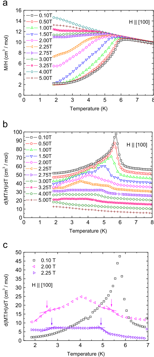
Fig. 3. (Color online) (a) M/H for different fields show antiferromagnetic behavior below the transition temperature for the lower fields. Between H=2 T and H=4 T different metamagnetic states are reached at the lowest temperatures and for field above 4.00 T no transition is seen. (b) We show d(MT/H)/dT to better highlight the transition temperatures [27]. Data for different temperatures have been shifted by 0.001 cm 3 /mol. (c) Detail of d(MT/H)/dT for some fields to show the types of features found in this derivatives and the criteria used for the selection of the transition temperatures. The H=2 T and the H=2.25 T data are shifted by 5 (cm 3 /mol) and -5 (cm 3 /mol) respectively for better visualization.
