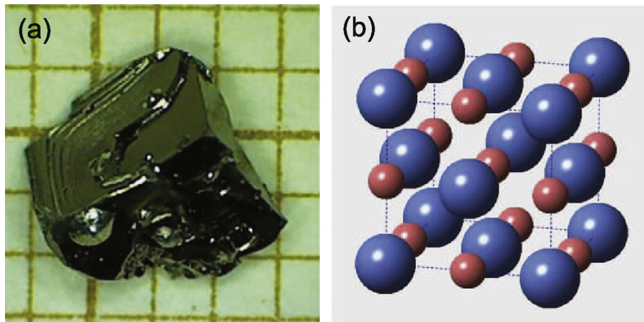
Fig. 1. (Color online) (a) HoBi crystal grown from an excess of Bi flux. Each of the small squares in the background corresponds to 1 mm. (b) Crystallographic structure of HoBi where blue (big) and red (small) spheres represent Ho and Bi ions respectively.
