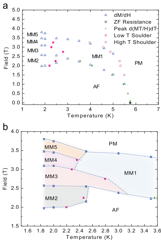
Fig. 5. (Color online) (a) In the H - T phase diagram several magnetic states can be differentiated. For low fields HoBi is paramagnetic (PM) down to T_N when it enters the antiferromagnetic (AF) phase. When higher external fields are applied up to five metamagnetic (MM) states appear. (b) Detail of the lower temperatures phase diagram. Lines are guides to the eye.
