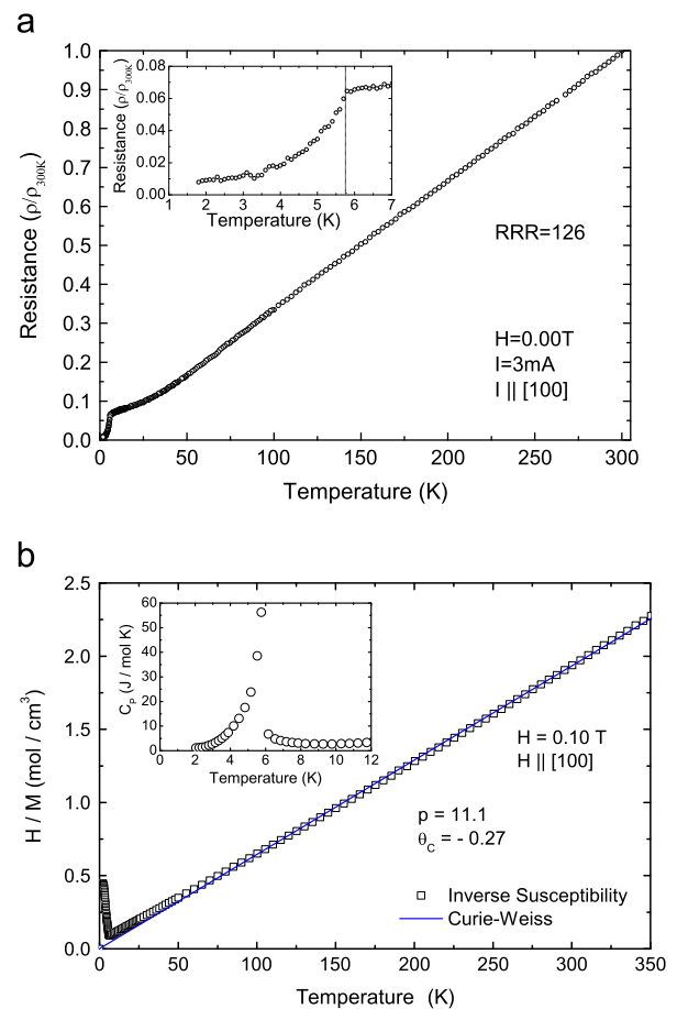
Fig. 2. (Color online) In (a) we show the temperature dependence of the resistance normalized to its ambient temperature value at zero magnetic field. Current is applied along the a axis of the cubic structure. In (b) we show the temperature dependence of the inverse susceptibility with a magnetic field of 0.1 T applied along the a axis. Blue line is a fit to the expression given in the text between 55 K and 350 K. Inset: Zero field specific heat shows a jump at the magnetic transition.
