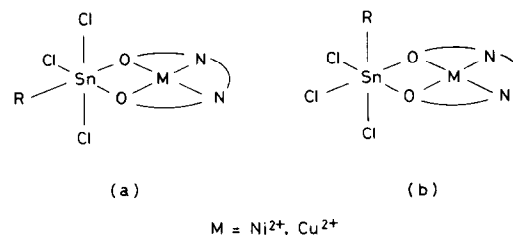
Fig. 2. Structure of organotin adducts.
