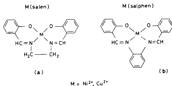
Fig. 1. Structures of \text{M}(\text{salen}) and \text{M}(\text{salphen}) .
