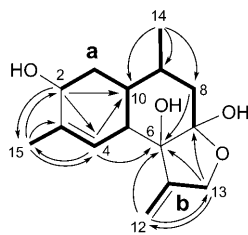
Fig. 1. Important ^1\text{H},^1\text{H} -COSY (bold lines) and HMBC (arrows) correlations observed for 5
