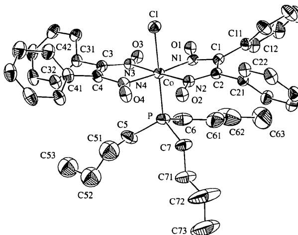
Fig. 1. ORTEP (Johnson, 1976) diagram of the molecule showing the labelling of the non-H atoms with 30% probability displacement ellipsoids. The ring C atoms are labelled Cij, where i = 1–4 and j = 1–6.
