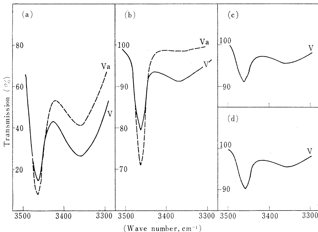
Fig. 2. Infrared Absorption Curves of N-(2-Cyanoethyl)-3-benzyloxycarbonylamino-cyclopentanecarboxamide (V), (solid line) and Its Epimer (Va), (broken line): (a) 0.064\text{ mole/liter} (Path length, 1\text{ mm} ), (b) 0.0064\text{ mole/liter} ( 1\text{ mm} ), (c) 0.00076\text{ mole/liter} ( 5\text{ mm} ), (d) 0.0038\text{ mole/liter} ( 1\text{ mm} )
