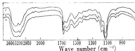
Fig. 1. Infrared Spectra (in 0.25% KBr disk) of (a) Myxoviomycine-sulfate, (b) dl -N-(2-Amidinoethyl)-3-aminocyclopentanecarboxamide (I), -sulfate (c) Its Epimer (Ia)-sulfate
