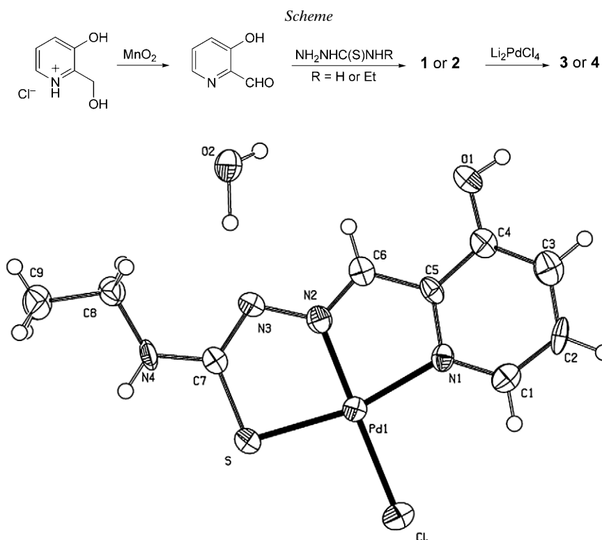
Fig. 2. X-Ray crystal structure of the \text{Pd}^{\text{II}} complex 4
