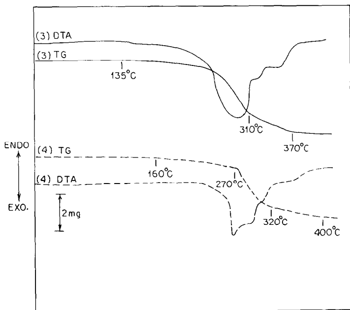
Fig. 2. Thermal curves of [\text{MnL}_2\text{Br}_2] (3) and [\text{MnL}_2\text{Br}_2] (4). Sample mass: complex (3), 19.73 mg; complex (4), 15.28 mg.
