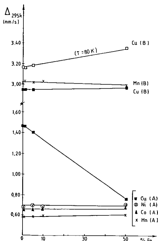
Fig. 4. Quadrupole splitting values of ^{57}\text{Fe}^{2+} in sites A and B against the composition of the mixed \text{Fe(II)}-\text{M(II)} dihydrated formates ( M = \text{Mn, Co, Ni, Cu} ).
