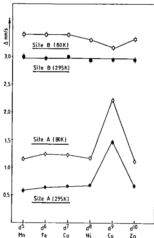
Fig. 5. Quadrupole splitting values of ^{57}\text{Fe}^{2+} ions at 295 K and 80 K in ^{57}\text{Fe} -doped (0.25 or 0.5 at.%) \text{M}(\text{HCO}_2)_2 \cdot 2\text{H}_2\text{O} .
