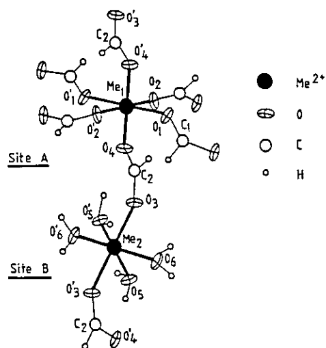
FIG. 1. Crystal structure of diaquadiformato compounds M^{II}(\text{HCO}_2)_2 \cdot 2\text{H}_2\text{O} with M = \text{Mn}, \text{Fe}, \text{Co}, \text{Ni}, \text{Cu}, \text{Zn} (from Ref. (8)).
