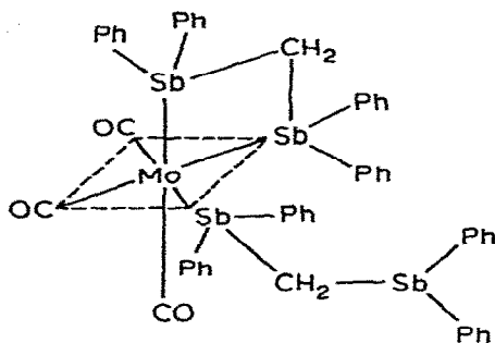
Fig. 3. Molecular structure of \text{Mo(CO)}_3(\text{Dpsm})_2 .
