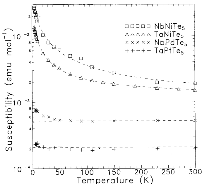
FIG. 6. Plots of molar magnetic susceptibility vs temperature for NbNiTe 5 , TaNiTe 5 , NbPdTe 5 , and TaPtTe 5 at 5 kG. For NbNiTe 5 and TaNiTe 5 , the dotted lines result from fits to the Curie-Weiss expression.
