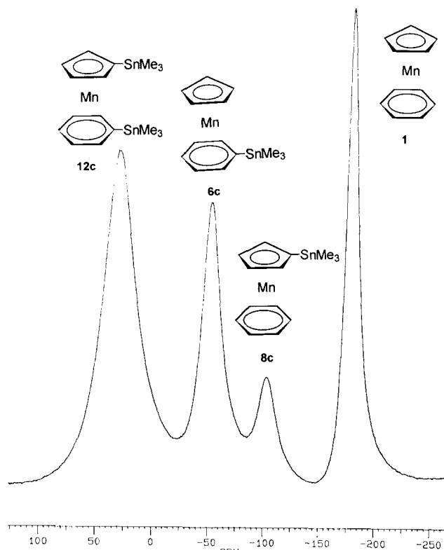
Fig. 1. 123.5 MHz ^{55}\text{Mn} NMR spectrum of a mixture of the sandwich complexes 1 , 6c , 8c and 12c , which is formed in the reaction of incompletely lithiated ( \eta^5 -cyclopentadienyl)manganese( \eta^6 -benzene) ( 1 ) with trimethyltin chloride.
