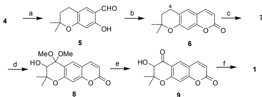
Scheme 2. Reagents and conditions: (a) 2-methyl-3-buten-2-ol, HCO 2 H, reflux, 4h, 57%; (b) Ph 3 P=CHCO 2 Et, Et 2 NPh, reflux, 0.5 h, 82%; (c) ceric ammonium nitrate, Et 2 O–AcOH–H 2 O, water bath, 30 min, 72%; (d) PhI(OAc) 2 , KOH, MeOH, rt, 20 h; (e) 3 M HCl, MeOH, rt, 30 min, 64% for two steps; (f) senecioid chloride, pyridine, CH 2 Cl 2 , rt, 3 h, 96%.
