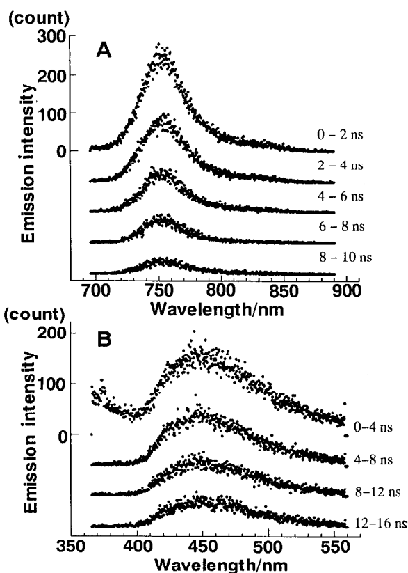
Figure 2. Time-resolved fluorescence (A) S_1 and (B) S_2 spectra of \text{Li}_2\text{Fluc} in deaerated DMF. The excitation was at 646 and 337 nm for the S_1 and S_2 emission, respectively.
