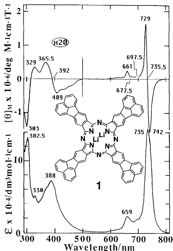
Figure 1. Electronic absorption (bottom) and magnetic circular dichroism spectra (top) of Li 2 Fluc in DMF. The inset shows the structure of Li 2 Fluc.
