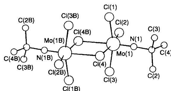
Fig. 1 Molecular structure of [\{\text{MoCl}_3(\mu\text{-Cl})(\text{NBu}^t)\}_2] 7 . Hydrogen atoms omitted for clarity
