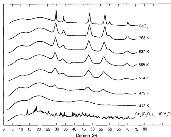
Fig. 3. X-ray powder diffraction patterns of hydrated cerous oxalate and its calcination products at various temperatures.
