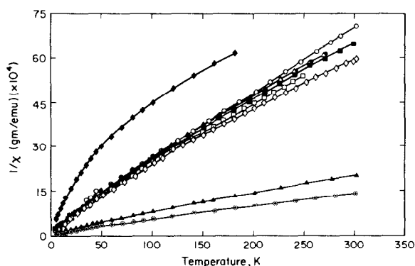
Fig. 4. Temperature dependence of the magnetic susceptibility of the various calcination products. Curves are shown for material heated at 412 K (○), 475 K (▲), 515 K (□), 563 K (■), 585 K (△), 613 K (◊), 637 K (●), and 810 K (◇). Data obtained for reagent grade ceric oxide (◆) are also included for comparison purposes.
