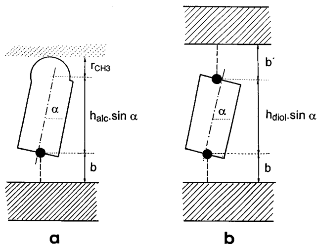
Figure 2. The basic idea about steric demands of 1-alkanol (a) and 1, \omega -diol (b) molecules for necessary gapping of rigid layers of host.
