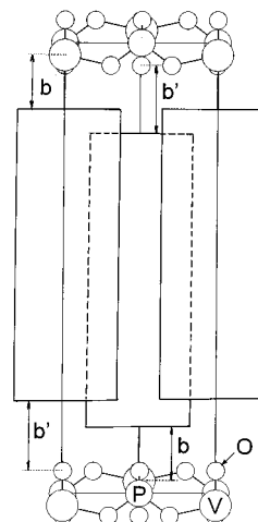
Figure 6. The principles of location of 1, \omega -alkanediol molecules in the interlayer space of the VOPO 4 host. The diol molecules are anchored to the layers by the same bonds as in the case of 1-alkanols.
