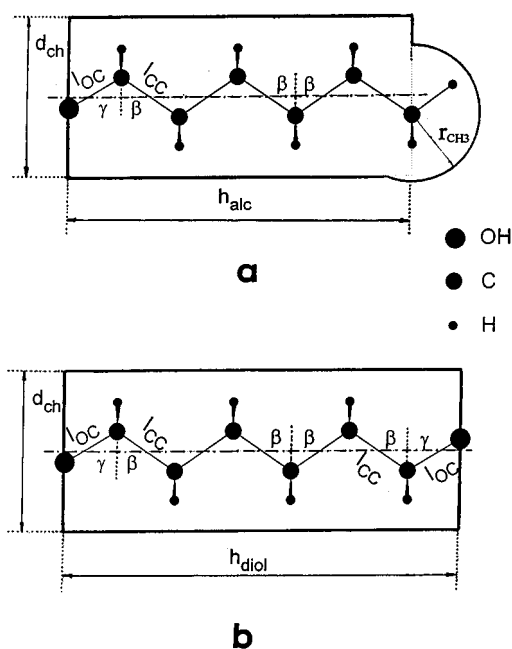
Figure 1. Representation of simplified shape and dimensions of molecules of 1-alkanols (a) and 1, \omega -diols (b). All of the aliphatic chains assume all-trans configurations.
