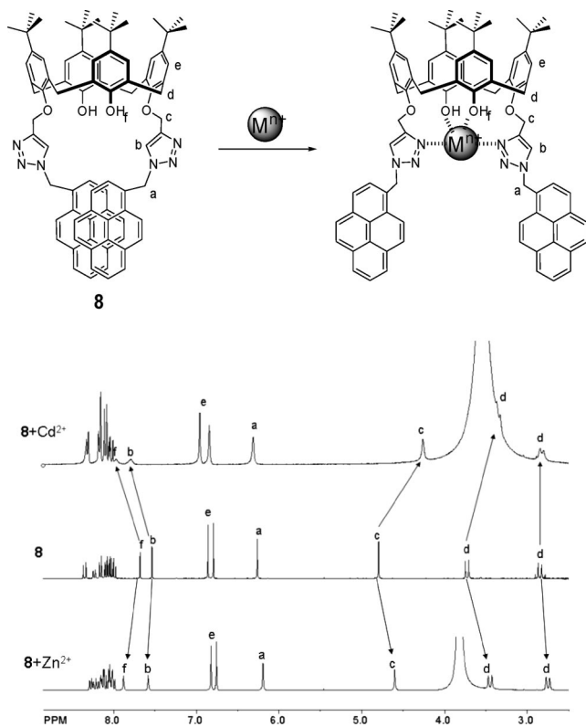
FIGURE 6. The proposed structure for 8 + metal ions, and ^1\text{H} NMR spectra of 8 in \text{CD}_3\text{CN} and in the presence of \text{Cd}(\text{ClO}_4)_2 and \text{Zn}(\text{ClO}_4)_2 in a 1:1 ratio (full spectra are available in the Supporting Information, Figures S17 and S18)
