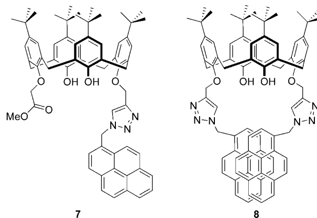
FIGURE 1. Structures of fluorescent sensors 7 and 8.
