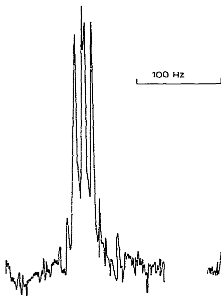
Fig. 3. ^{19}\text{F} NMR spectrum of complex II.
