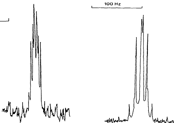
Fig. 4. ^{19}\text{F} NMR spectrum of complex III.
