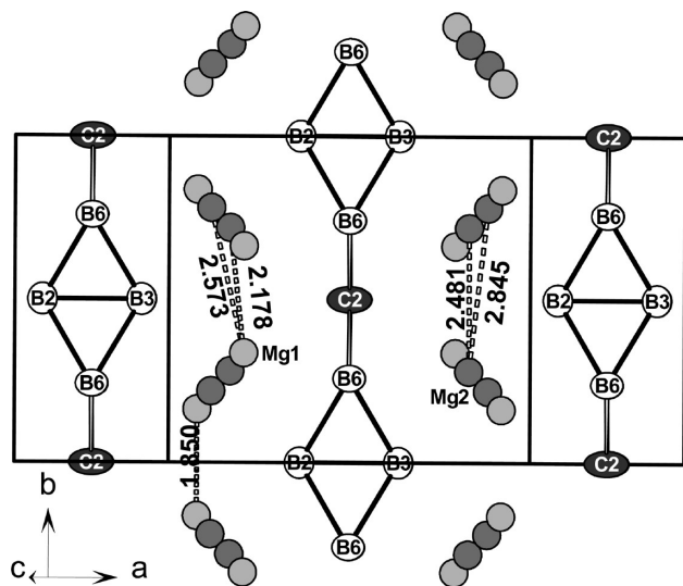
Figure 6. Structure of Mg 3 B 50 C 8 at z ≈ 0.5.
