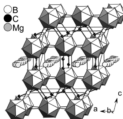
Figure 2. Crystal structure of \text{Mg}_3\text{B}_{50}\text{C}_8 .
