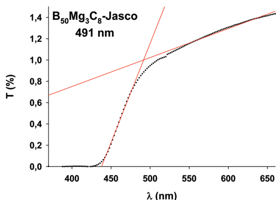
Figure 9. UV-vis spectrum in transmission of a Mg 3 B 50 C 8 single crystal.
