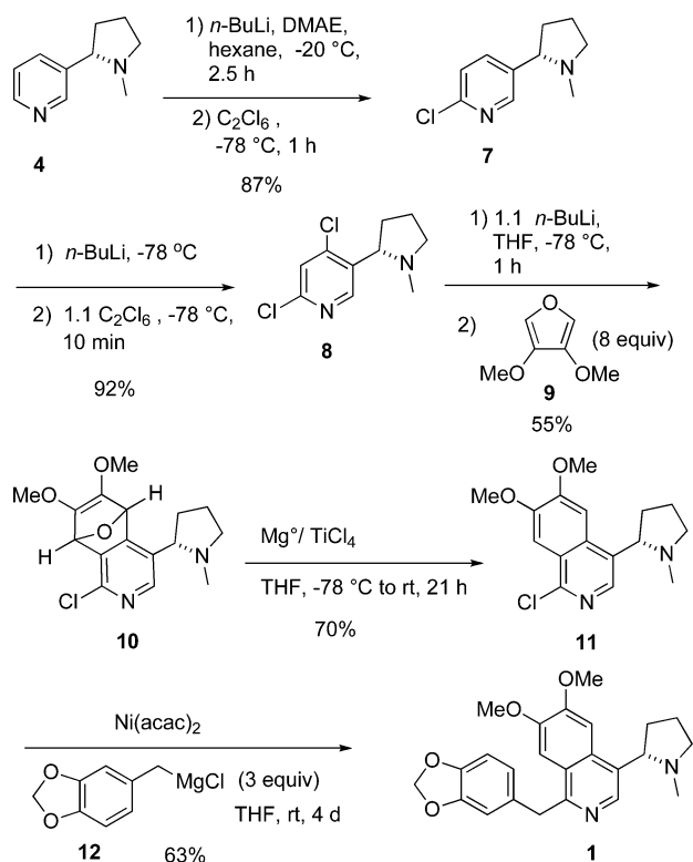
Scheme 2. Synthesis of ( S )-Macrostomine ( 1 ) from ( S )-Nicotine
