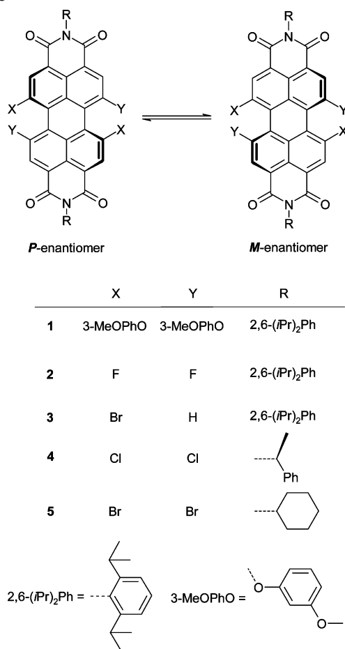
Scheme 1. Racemization Equilibrium and Structures of Bay-Substituted Perylene Bisimides 1–5 Used in the Present Investigation
