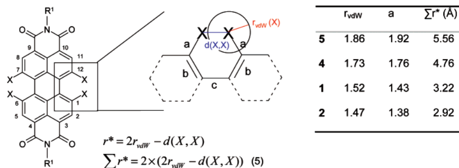
Figure 5. Definition of geometrical parameters for 1,6,7,12-tetrasubstituted perylene bisimides and the equations necessary for the calculation of the apparent overlap \sum r^* . The table (right) summarizes the apparent overlap values for PBIs 1, 2, 4, and 5 (ordered according to decreasing overlap value). The apparent overlap of 1 was calculated for a hypothetical PBI bearing only oxygen atoms in the bay positions. For the calculation of apparent overlap values for 1,7-substituted PBIs, see the Supporting Information.
