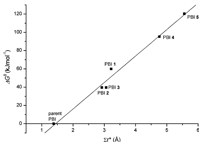
Figure 6. Dependence of the free activation enthalpy of racemization on the apparent overlap \sum r^* for PBIs 1–5 (data are taken from Table 2 and Figure 5).
