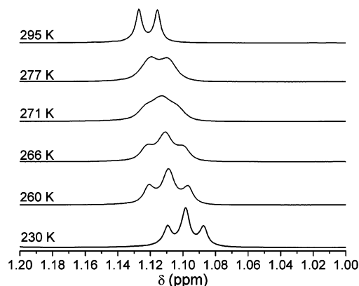
Figure 1. Sections of the temperature-dependent 1 H NMR spectra of 1 (600 MHz) in CDCl 3 . The signals of the diastereotopic methyl groups of the diisopropylphenyl imide substituents are shown.
