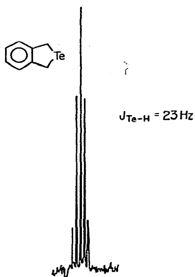
Fig. 1. ^{125}\text{Te} NMR spectrum of C_8H_8Te in CDCl_3 . 100 transients; 3.6 sec delay, no proton decoupling.
