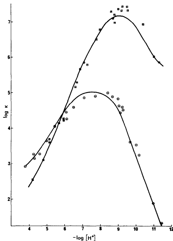
Figure 1. Plot of the observed rate constants for reaction of CuPAPHY with trien \square and EDTA \odot as a function of hydrogen ion concentration. The solid lines are calculated on the basis of the resolved rate constants in Table III.
