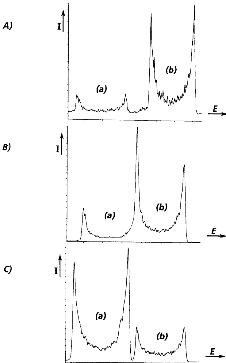
Fig. 1. Partial MIKE spectra of [\text{MC}_{10}\text{H}_{10}]^{2+} dications generated from (A) ferrocene, (B) cobaltocene and (C) nickelocene, showing charge separation reactions (a) and (b) (see Scheme 2).
