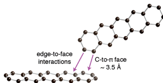
Figure 4. Crystal structure of tetraphenyl pentacene, 3 . Phenyl side chains and the hydrogens have been suppressed in this view. The magenta arrows show close contacts between the edge of one acene and the face of another.
