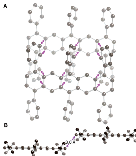
Figure 5. Crystal structure of hexaphenyl pentacene, 4 : (A) magenta arrows showing the 12 close contacts (approximately 3.8 Å C-to-C) between the phenyl side chains and the acene core; (B) 3.6 Å separates the ends of the acenes (shown with a magenta arrow). Hydrogens have been removed to clarify the view.
