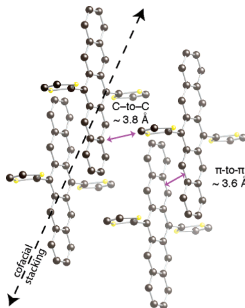
Figure 7. Crystal structure of 6,13-di(2'-thienyl)pentacene, 2b , showing a cofacial, one-dimensional stack. The magenta arrows show the close contacts between the acene faces and neighboring columns. The position of the sulfur atoms (yellow balls) is disordered in the crystal.
