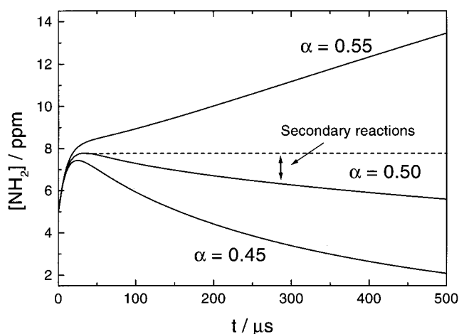
Figure 1. Solid lines: CHEMKIN simulations of \text{NH}_2 mole fraction time profiles for three different values of the branching ratio, \alpha , and typical experimental conditions of this study: [\text{NH}_3] = 1\% , [\text{NO}] = 0.2\% , [\text{H}]_0 = [\text{NH}_2]_0 = 5 ppm, T = 1500 K, p = 1.3 atm. Dashed line: eq 10 for the same conditions.
