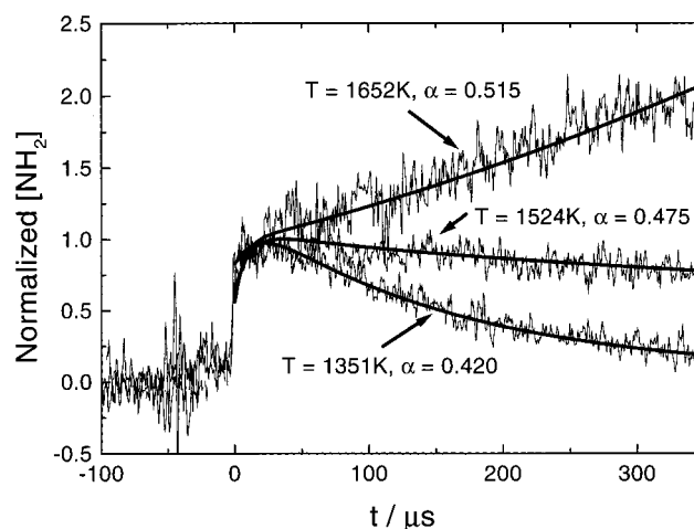
Figure 3. Thin lines: normalized \text{NH}_2 concentration time profiles for three different temperatures. Experimental conditions: [\text{NH}_3] = 1\% , [\text{NO}] = 0.2\% , p \approx 1.3 atm. One arbitrary concentration unit corresponds to \text{NH}_2 mole fractions of 5.5, 7.3, and 4.8 ppm at 1351, 1524, and 1652 K, respectively. Bold lines: CHEMKIN fits with \alpha as a single fit parameter.
