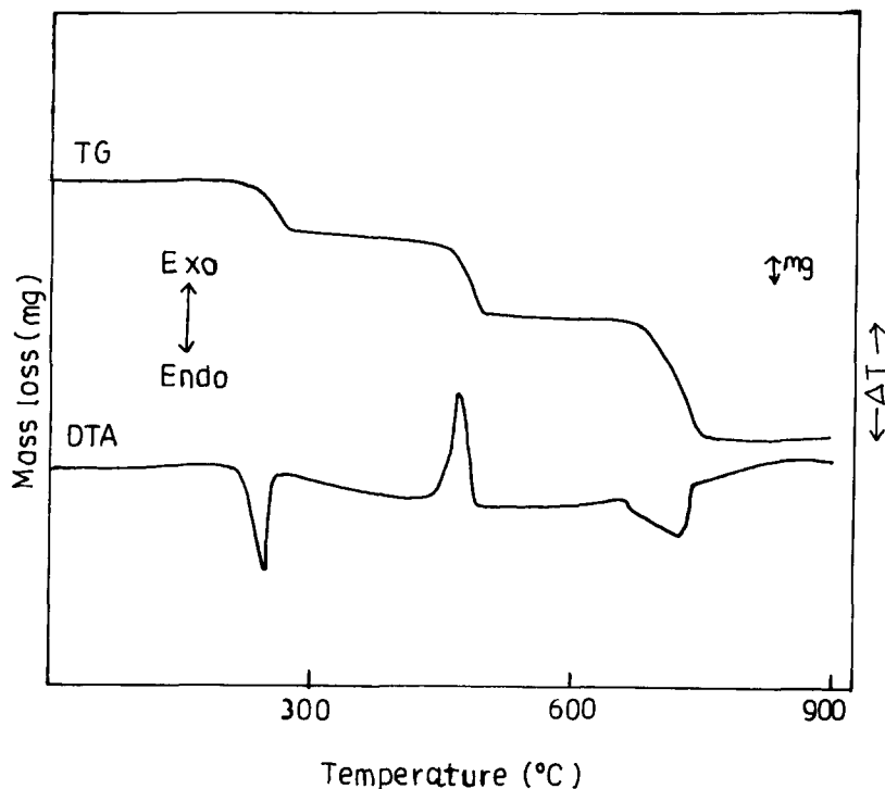
Fig. 1. Simultaneous TG-DTA curve of pure \text{CaOx} \cdot \text{H}_2\text{O} . 10 mg sample, static air, rate of heating, 10^\circ\text{C min}^{-1} .
