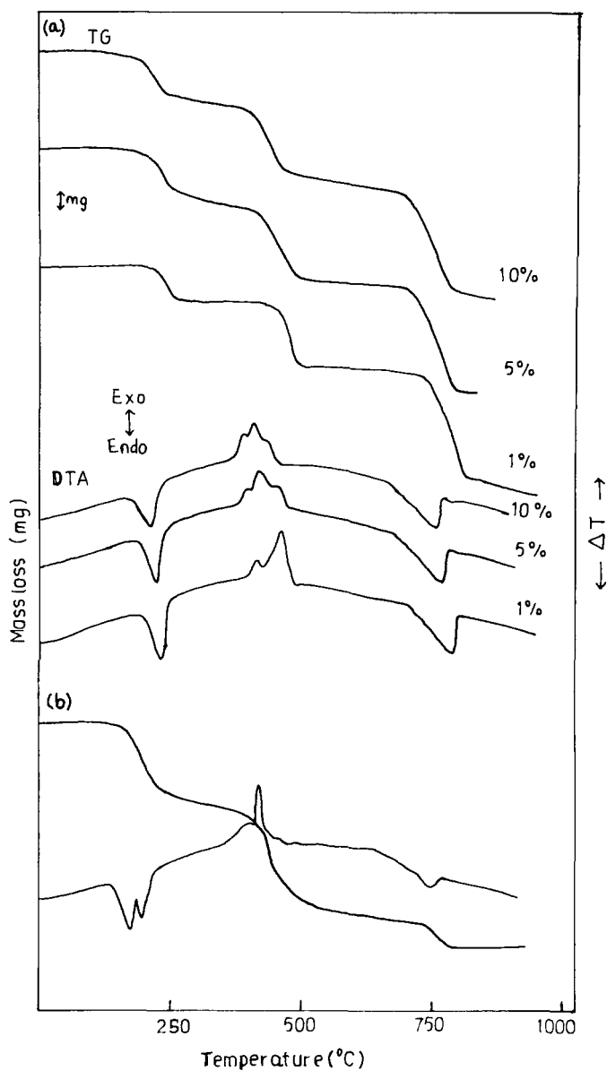
Fig. 2. Simultaneous TG-DTA curve of: (a) CaOx doped with 1%, 5% and 10% La; (b) pure \text{La}_2(\text{C}_2\text{O}_4)_3 \cdot 10\text{H}_2\text{O} . 15 mg sample, static air, rate of heating, 10^\circ\text{C min}^{-1} .
