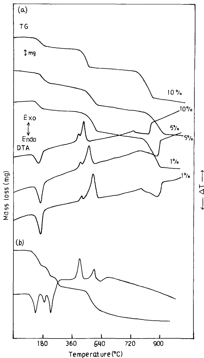
Fig. 4. Simultaneous TG-DTA curve of: (a) CaOx doped with 1%, 5% and 10% Gd; (b) pure \text{Gd}_2(\text{C}_2\text{O}_4)_3 \cdot 10\text{H}_2\text{O} . 10 mg sample, static air, rate of heating, 10^{\circ}\text{C min}^{-1} .
