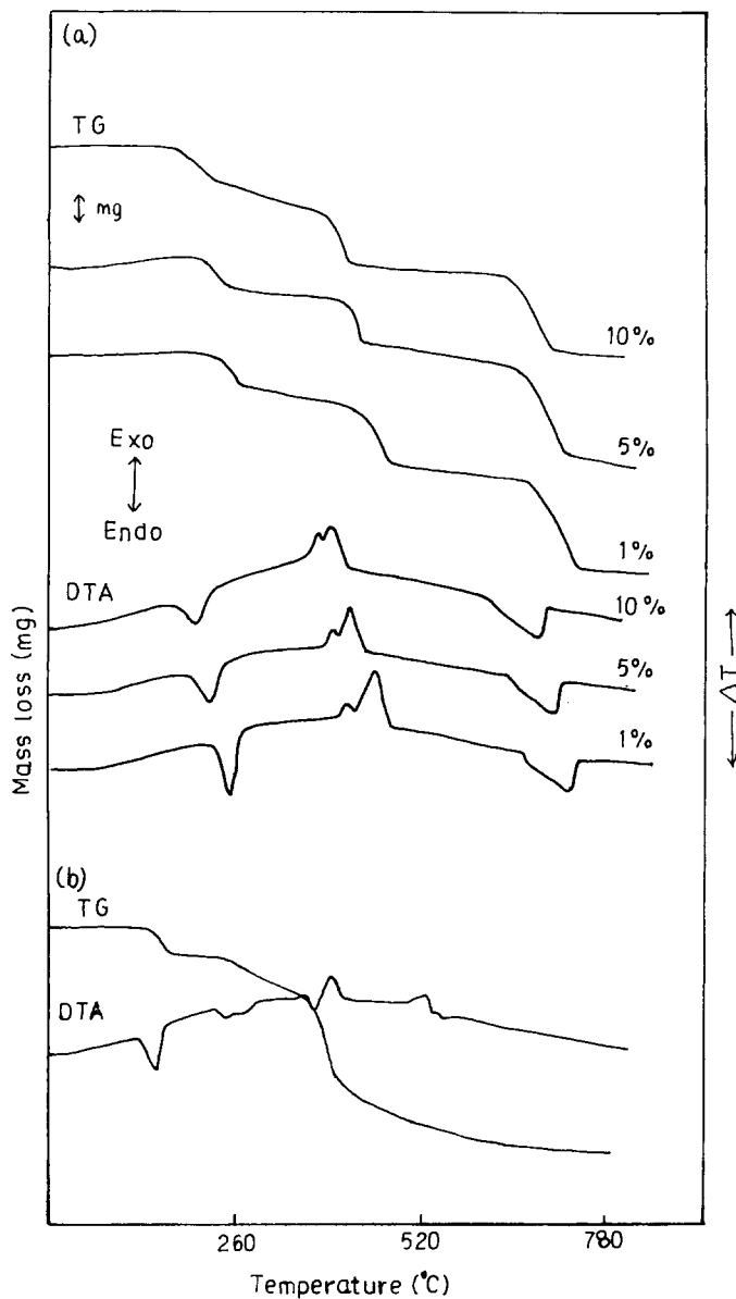
Fig. 3. Simultaneous TG-DTA curve of: (a) \text{CaOx} doped with 1%, 5% and 10% Sm; (b) pure \text{Sm}_2(\text{C}_2\text{O}_4)_3 \cdot 10\text{H}_2\text{O} . 10 mg sample, static air, rate of heating, 10^\circ\text{C min}^{-1} .
