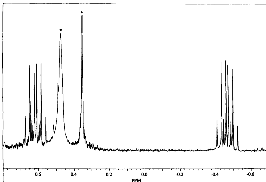
Fig. 3. The \text{ReEt} \alpha -hydrogen region of the ^1\text{H} NMR spectrum of \text{Re}(\text{Et})(\text{CO})_3(^i\text{Pr-pyCa}) (benzene- d_6 , 300 MHz) (* denotes contaminant in the solvent).
