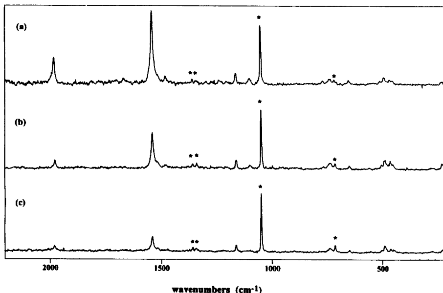
Fig. 5. Resonance Raman spectra of \text{Re}(\text{Me})(\text{CO})_3(^i\text{Bu-DAB}) in a \text{KNO}_3 disk at room temperature (a) \lambda_{\text{exc}} = 457.9 \text{ nm} , (b) \lambda_{\text{exc}} = 514.5 \text{ nm} and (c) \lambda_{\text{exc}} = 533.5 \text{ nm} (* = \text{KNO}_3 ).
