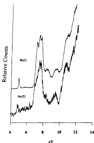
Fig. 7. \text{He}^I and \text{He}^{II} photoelectron spectra of \text{Re}(\text{Me})(\text{CO})_3(^i\text{Pr-DAB}) .
