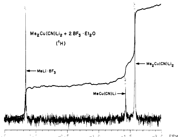
Figure 1. Proton NMR spectrum of Me 2 Cu(CN)Li 2 + 2BF 3 ·Et 2 O in THF at -92 °C.
