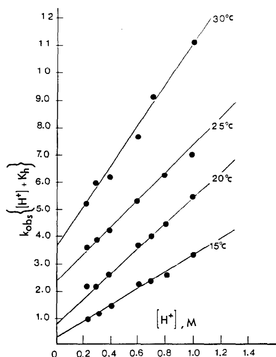
Fig. 2. [\text{H}^+] dependence. Plot of k_{\text{obs}} ([\text{H}^+] + K_h) vs. [\text{H}^+] ( \mu = 1.0 \text{ M (HCl/NaCl)}, T = 25.0^\circ\text{C} ).
