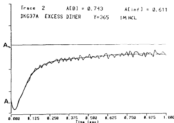
Fig. 1. Stopped-flow kinetic trace. [Dimer]_0 = 8.17 \times 10^{-3} M, [VO_2^+]_0 = 0.80 \times 10^{-3} M ( [H^+] = \mu = 1.0 M ( HCl ), T = 25.0^\circ C ).
