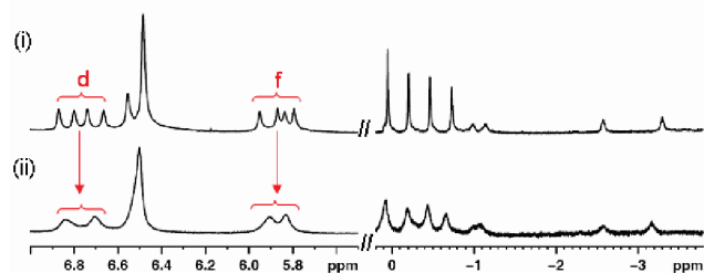
Figure 4. Partial ^1\text{H} NMR spectra (400 MHz, \text{D}_2\text{O} ) of \mathbf{2a@OA_2} ( [\text{OA}] = 1 \text{ mM} , [\mathbf{2a}] = 0.5 \text{ mM} , in 10 mM sodium tetraborate buffer) at (i) 25 °C and (ii) 70 °C.
