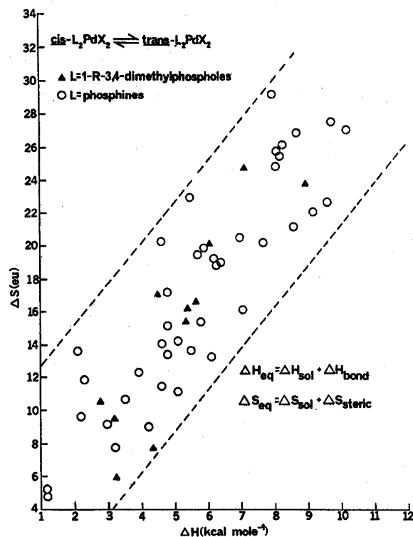
Figure 1. Plot of \Delta S vs. \Delta H for Pd(II) compounds of the type L_2PdX_2 where X = Cl^- , N_3^- , or Br^- . Data taken from this work and ref 19 and 29 ( \blacktriangle ) represent the (1-R-3,4-dimethylphosphole)palladium(II) complexes.
