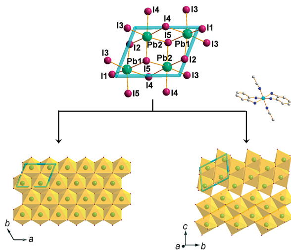
Figure 2. Cation effect leading to symmetry breaking. Left: single hcp layer in \text{PbI}_2 . Right: single [\text{Pb}_4\text{I}_{10}]^n_- anionic layer in 1 . The blue rhombus confines the 2 \times 2 subunit.
