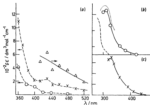
FIGURE 1 Absorption spectra of intermediates formed in aqueous iron(II) sulphate solutions. (a) Argon-saturated solutions: 3 \times 10^{-3} \text{ mol dm}^{-3} \text{ Fe}[\text{SO}_4] , pH 2.65 (O); 0.4 \text{ mol dm}^{-3} \text{ Fe}[\text{SO}_4] , pH 3.65, measured 5 \mu\text{s} after the pulse (x); spectrum of \text{Fe}^+ intermediate ( \Delta ). Absorbed dose 7.7 krad. (b) \text{N}_2\text{O} -saturated 3 \times 10^{-3} \text{ mol dm}^{-3} \text{ Fe}[\text{SO}_4] , pH 3.2, measured 600 \mu\text{s} after pulse (O). Absorbed dose 6.9 krad. Broken and dotted lines represent the spectra of \text{Fe}^{3+} and [\text{Fe}(\text{SO}_4)]^+ , respectively, taken from ref. 10. (c) Argon-saturated 4 \times 10^{-2} \text{ mol dm}^{-3} \text{ Fe}[\text{SO}_4] , pH 0.55. Absorbed dose 6.9 krad.
