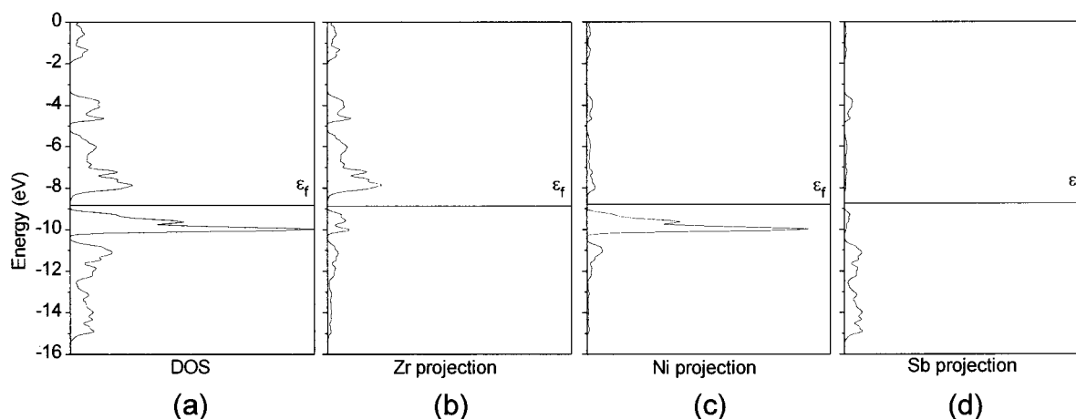
Figure 3. (a) Total density of states (DOS) curve for \text{Zr}_3\text{Ni}_3\text{Sb}_4 and its (b) Zr, (c) Ni, and (d) Sb projections.
