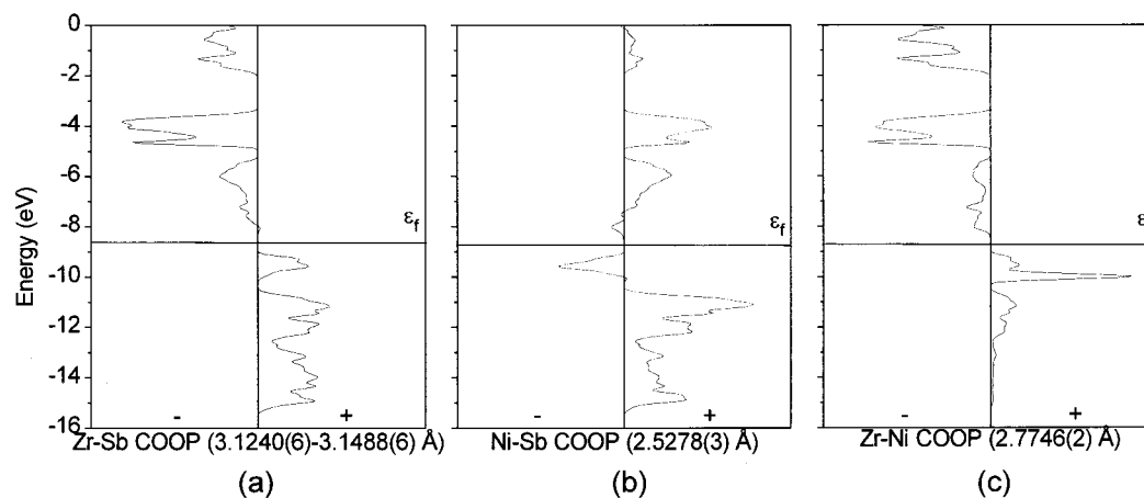
Figure 4. Crystal orbital overlap population (COOP) curves for (a) Zr–Sb, (b) Ni–Sb, and (c) Zr–Ni contacts in \text{Zr}_3\text{Ni}_3\text{Sb}_4 .
