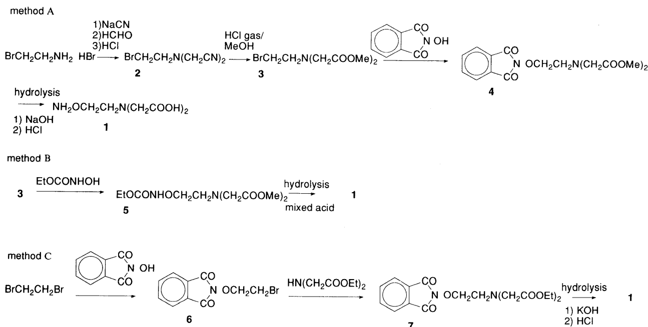
Chart 1. Syntheses of 2-Aminooxyethyliminodiacetic Acid ( 1 )
