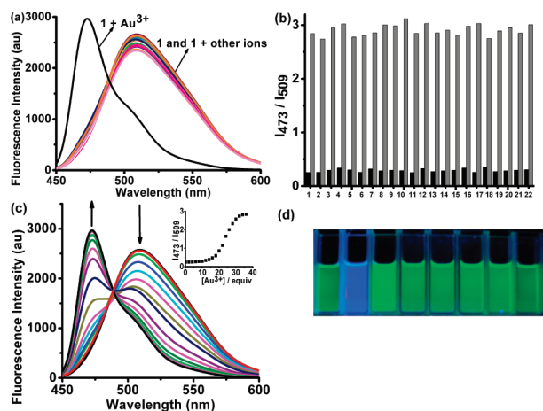
Figure 3. (a) Fluorescence responses of 1 (5 \mu\text{M} ) with various metal ions (180 \mu\text{M} ) in \text{MeOH-H}_2\text{O} (95:5 v/v, pH = 9.0) ( \lambda_{\text{ex}} = 420 nm). (b) Metal-ion selectivity of 1 (5 \mu\text{M} ). The black bars represent the emission intensity of 1 in the presence of other cations (500 \mu\text{M} ). The gray bars represent the emission intensity that occurs upon the subsequent addition of 180 \mu\text{M} \text{Au}^{3+} to the above solution. From 1 to 21: none, \text{Ag}^{+} , \text{Au}^{+} , \text{Al}^{3+} , \text{Ba}^{2+} , \text{Ca}^{2+} , \text{Cd}^{2+} , \text{Co}^{2+} , \text{Cu}^{2+} , \text{Fe}^{2+} , \text{Fe}^{3+} , \text{Hg}^{2+} , \text{K}^{+} , \text{Li}^{+} , \text{Mg}^{2+} , \text{Mn}^{2+} , \text{Na}^{+} , \text{Ni}^{2+} , \text{Pb}^{2+} , \text{Sr}^{2+} , \text{Zn}^{2+} , and \text{Pd}^{2+} . (c) Fluorescent spectra of 1 (5 \mu\text{M} , \text{MeOH-H}_2\text{O} , 95:5 v/v, pH = 9.0) upon addition of \text{Au}^{3+} (0–36.0 equiv) ( \lambda_{\text{ex}} = 420 nm). Inset: Ratiometric fluorescence intensity [ I_{473}/I_{509} ] as a function of [\text{Au}^{3+}] . (d) Fluorescence change of 1 . Left to right: 1 only, \text{Au}^{3+} , \text{Hg}^{2+} , \text{Zn}^{2+} , \text{Cd}^{2+} , \text{Cu}^{2+} , \text{Ag}^{+} , \text{Pb}^{2+} .
