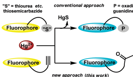
Scheme 1. Reaction-Based Tactics for the Sensing of Hg 2+
