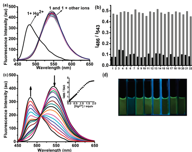
Figure 1. (a) Fluorescence responses of 1 (5 \mu\text{M} ) with various metal ions (10 \mu\text{M} ) in HEPES buffer (0.01 M, pH = 7.4) (0.05% DMSO, v/v) ( \lambda_{\text{ex}} = 420 nm). (b) Metal-ion selectivity of 1 (5 \mu\text{M} ). The black bars represent the emission intensity of 1 in the presence of other cations (5 \mu\text{M} ). The gray bars represent the emission intensity that occurs upon the subsequent addition of 0.6 \mu\text{M} \text{Hg}^{2+} to the above solution. From 1 to 21: none, \text{Ag}^+ , \text{Au}^{3+} , \text{Au}^+ , \text{Al}^{3+} , \text{Ba}^{2+} , \text{Ca}^{2+} , \text{Cd}^{2+} , \text{Co}^{2+} , \text{Cu}^{2+} , \text{Fe}^{2+} , \text{Fe}^{3+} , \text{K}^+ , \text{Li}^+ , \text{Mg}^{2+} , \text{Mn}^{2+} , \text{Na}^+ , \text{Ni}^{2+} , \text{Pb}^{2+} , \text{Sr}^{2+} , \text{Zn}^{2+} , and \text{Pd}^{2+} . (c) Fluorescent spectra of 1 (5 \mu\text{M} ) upon addition of \text{Hg}^{2+} ( \lambda_{\text{ex}} = 420 nm). Inset: Ratiometric fluorescence intensity [ I_{486}/I_{543} ] as a function of [ \text{Hg}^{2+} ]. (d) Fluorescence change of 1 . Left to right: 1 only, \text{Hg}^{2+} , \text{Zn}^{2+} , \text{Cd}^{2+} , \text{Cu}^{2+} , \text{Ag}^+ , \text{Au}^{3+} , \text{Pb}^{2+} .
