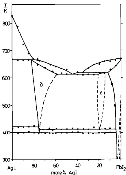
Fig. 1. The system AgI– \text{PbI}_2 .
