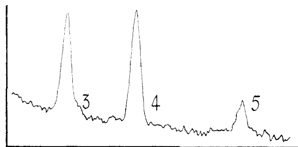
Fig. 3.—Raman spectrum for silicon chloriodides: \text{SiCl}_3\text{I} + \text{HI} at 325^\circ .
