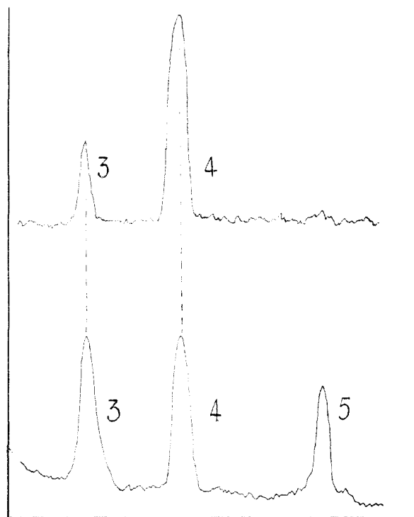
Fig. 2.—Raman spectra for silicon chloriodides: (A) upper, \text{SiCl}_3\text{I} at 325^\circ ; (B) lower, \text{SiCl}_3\text{I} at 400^\circ .
