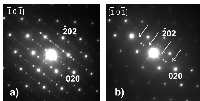
Figure 4. Electron diffraction pattern of (a) a crystal of \text{P}'3\text{-Na}_{0.60}\text{VO}_2 presenting a modulation along the b^* axis and (b) its tilt of a few degrees. The tilt makes the reflections m = 1 and 3 disappear, which is in agreement with the superspace group C2/m(0\ \beta\ 0)\ s0 .
