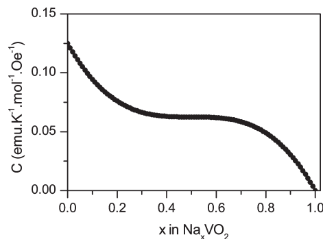
Figure 11. x value dependence of the theoretical C Curie constant by assuming a pseudotriangular cluster model where x is the composition in \text{Na}_x\text{V}^{3+}_x\text{V}^{4+}_{1-x}\text{O}_2 . The C Curie constant is calculated on the basis of the ground state of the total spin S_t = 1/2 : C_{th} = [(1-x)^3 + 3x^2(1-x)]/3 \times 0.375 .
