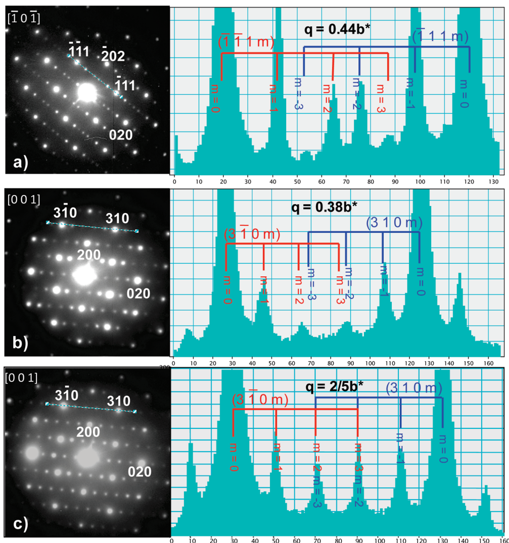
Figure 3. Electron diffraction pattern of three different crystals of \text{P}'3\text{-Na}_{0.60}\text{VO}_2 . The right part of the figure represents the intensity evolution along the [0\ 1\ 0]^* direction corresponding to the blue line in the pattern. The whole pattern can be indexed considering the cell parameters given in Table 1 and a vector q equal to (a) 0.44b^* , (b) 0.38b^* , and (c) 0.40b^* . The satellites are observed at least up to m = 3 .
