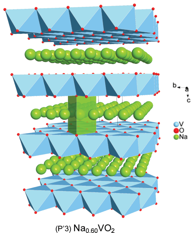
Figure 6. View of the structure of \text{P'3-Na}_{0.60}\text{VO}_2 . All \text{VO}_6 octahedra and only one \text{NaO}_6 trigonal prism are drawn.
