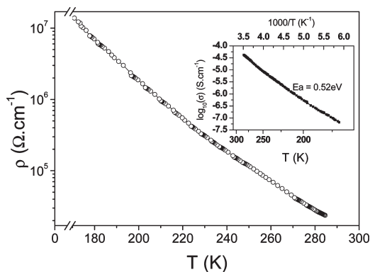
Figure 7. Temperature dependence of the electrical resistivity measured on sintered pellets for \text{P'3-Na}_{0.60}\text{VO}_2 between 170 and 300 K. The inset represents an Arrhenius plot of the conductivity versus reciprocal temperature. The activation energy has been deduced from the slope of the curve and is equal to 0.52 eV.
