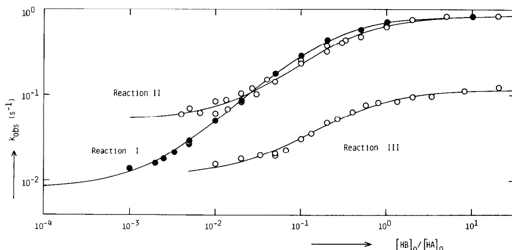
Fig. 1. Double logarithmic plot of k_{\text{obs}} vs. [\text{HB}]_o/[\text{HA}]_o for Reactions I–III (solid lines: calculated by computer fitting).
