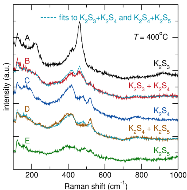
Figure 6. Raman spectra (same data as Figure 5) of \text{K}_2\text{S}_3 – \text{K}_2\text{S}_5 mixtures at T = 400^\circ\text{C} (solid lines), fit using linear combinations (dashed lines) of the \text{K}_2\text{S}_3 , \text{K}_2\text{S}_4 , and \text{K}_2\text{S}_5 spectra. The data can be reproduced by assuming that \text{K}_2\text{S}_4 has a distinct molten structure, as it does in the solid phase.
