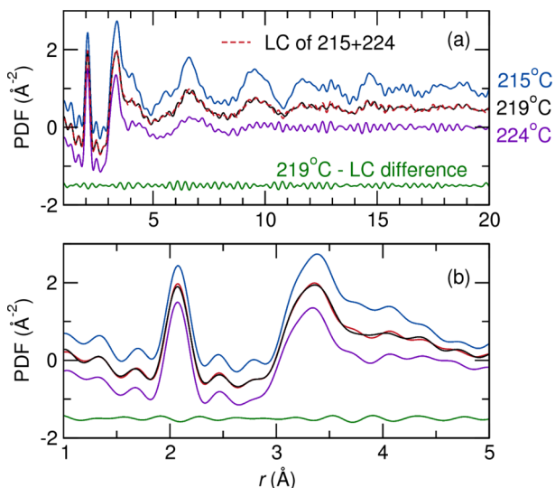
Figure 9. K_2S_5 PDF in the vicinity of melting, showing a loss of long-range structure from 215 to 224 °C. The linear combination (LC, dashed) of the 215 and 224 °C data reproduces the data from 219 °C, showing that K_2S_5 is congruently melting. Difference curve of the 219 °C data minus LC is shown below. Data curves offset by \pm 1 for clarity.
