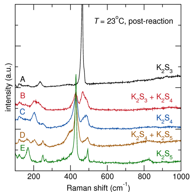
Figure 7. Raman spectra of the polysulfides after cooling, showing formation of \text{K}_2\text{S}_4 , and mixtures with \text{K}_2\text{S}_3 and \text{K}_2\text{S}_5 .
