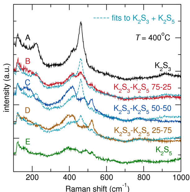
Figure 5. Raman spectra of \text{K}_2\text{S}_3 – \text{K}_2\text{S}_5 mixtures at T = 400^\circ\text{C} (solid lines), fit using linear combinations (dashed lines) of the \text{K}_2\text{S}_3 and \text{K}_2\text{S}_5 spectra. These fits of the type (c_A A + c_E E) do not reproduce the spectra for the mixed compositions, unlike before these samples were subjected to heating (Figure 4), implying that the distribution of \text{S}_n^{2-} is not smoothly varying across the series.
