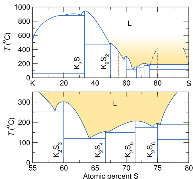
Figure 1. K–S phase diagram containing the low-melting compounds K_2S_3 ( T_m = 302\text{ }^\circ\text{C} ), K_2S_4 ( T_m = 154\text{ }^\circ\text{C} ), which is glassy, K_2S_5 ( T_m = 206\text{ }^\circ\text{C} ), and K_2S_6 ( T_m = 183\text{ }^\circ\text{C} ). Adapted from Sangster; 32 dotted region is shown as an inset in the bottom pane. The shaded region represents conditions where the low-melting flux may enable controlled growth of new materials.
