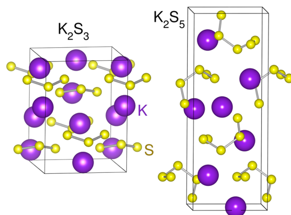
Figure 2. Unit cells of K_2S_3 ( Cmc2_1 , 7.31 \times 9.91 \times 7.47\text{ Å} ) and K_2S_5 ( P2_12_12_1 , 6.49 \times 6.60 \times 17.41\text{ Å} ) containing polysulfide chains of S_3^{2-} and S_5^{2-} respectively, shown here connected by bonds.
