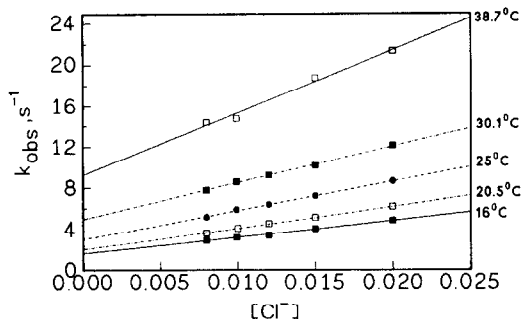
Fig. 4. Typical plots of k_{\text{obs}} vs. [\text{Cl}^-] for the reaction of \text{Pd}(\text{Me}_4\text{en})(\text{H}_2\text{O})\text{Cl}^+ with \text{Cl}^- as a function of temperature (data taken from Table 1).
