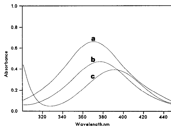
Fig. 1. UV-Vis spectra of \text{Pd}(\text{Et}_4\text{en}) complexes in aqueous solution. Experimental conditions: [\text{Pd}(\text{II})] = 1.0 \times 10^{-3} M; optical pathlength = 1.0 cm; pH \approx 3. (a) Solution of \text{Pd}(\text{Et}_4\text{en})(\text{H}_2\text{O})_2^{2+} , \lambda_{\text{max}} = 365\text{--}370 nm. (b) Equilibrated solution of \text{Pd}(\text{Et}_4\text{en})\text{Cl}_2 dissolved in water, \lambda_{\text{max}} = 375 nm. (c) After addition of large excess of solid \text{NaCl} to solution b, \lambda_{\text{max}} = 392 nm.
