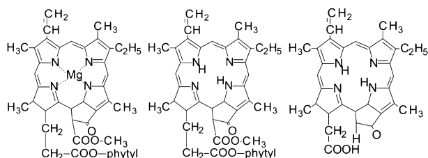
Chl a (MW 893.5) Pheo a (MW 871.1) Pyroside a (MW 534.7)
