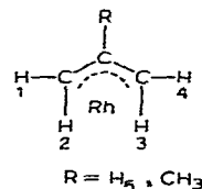
Fig. 1. The three possible configurations of L_2Cl_2Rh(\pi-C_3H_4R) and the one of [(Ph_3P)_2Pt(\pi-C_3H_5)]^+ Cl^- .
