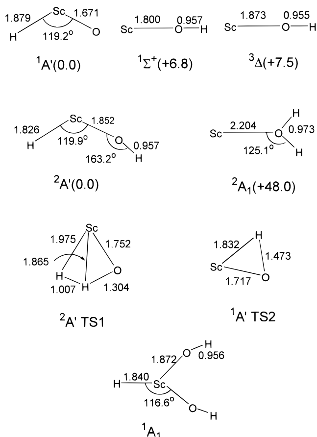
Figure 4. Calculated geometric parameters for the \text{Sc} + \text{H}_2\text{O} reaction products and transition states (bond length in Å, bond angle in degree, relative energies for different isomers are given in parentheses in kcal/mol).
