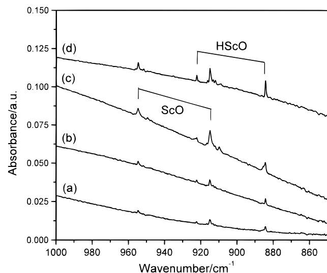
Figure 3. Infrared spectra in the 1000–850 \text{cm}^{-1} region from codeposition of laser-ablated Sc atoms with 0.1% \text{H}_2\text{O} + 0.4% \text{H}_2^{18}\text{O} in argon: (a) 1 h sample deposition at 11 K; (b) after 25 K annealing; (c) after 20 min \lambda > 250 nm photolysis; (d) after 30 K annealing.
